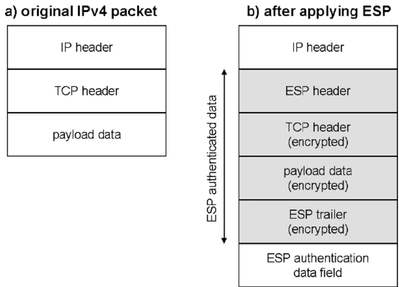
Figure 13.33 IPsec: encapsulating security payload (ESP) position and scope of the authenticated data.
