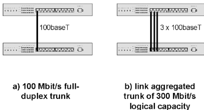
Figure 4.20 Interconnecting switches: port trunking and link aggregation.
