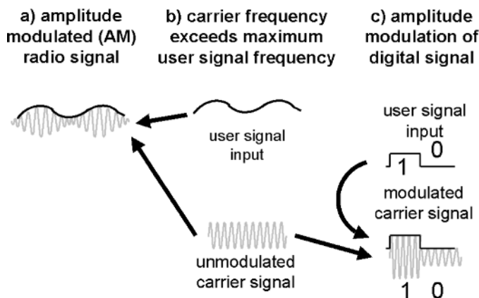
Figure 2.5 Amplitude modulation (AM).
