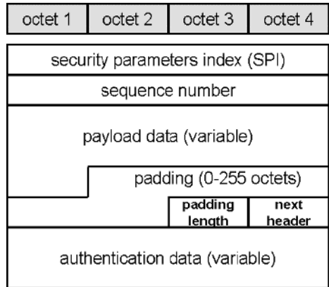
Figure 13.32 IPsec: encapsulating security payload (ESP) format of IP packet contents (RFC 2406).
