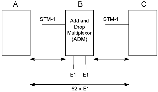
Figure 3.15 Add/drop multiplexor (ADM) used to break-out 2 Mbit/s (E1) from a 155 Mbit/s (STM-1) line.
