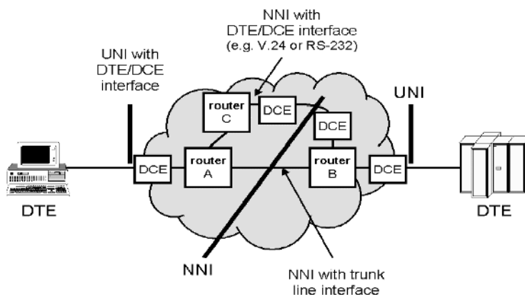
Figure 3.3 DTE/DCE Interface and Trunk or line interface.
